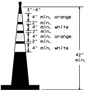
Two-Piece cones
